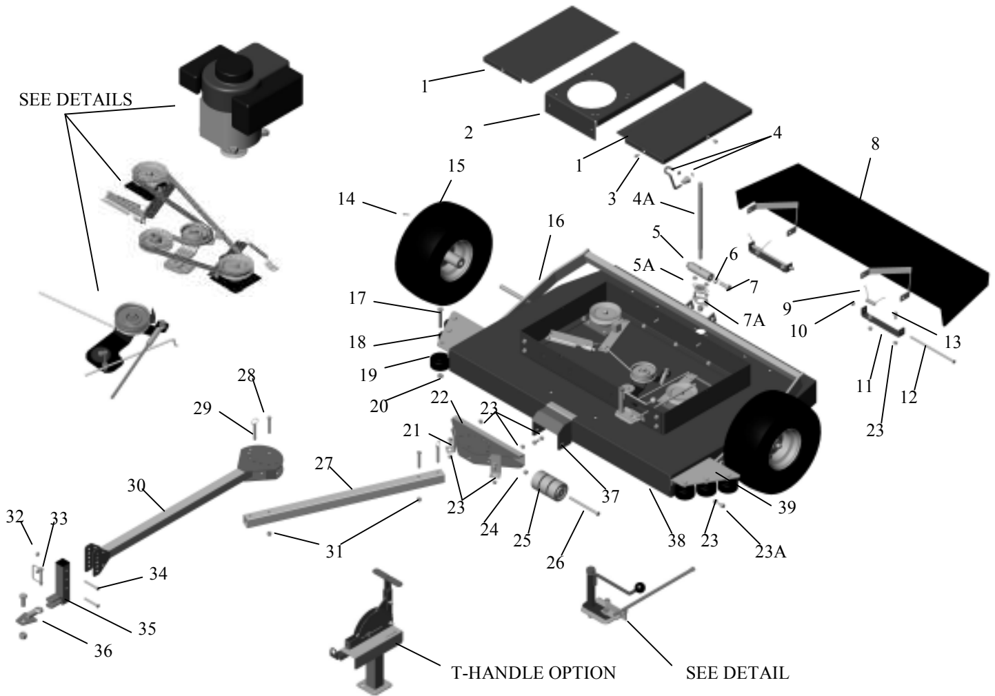
FIGURE FOUR SINGLE POINT HEIGHT ADJUST
